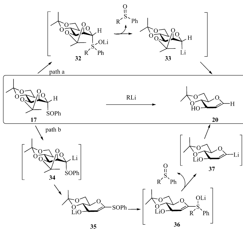
Scheme 8. Possible pathways for the transformation of sulfoxide 17 into glycal 20 mediated by organolithium reagents.
