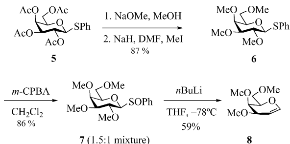
Scheme 2. Preparation of galactal derivative 8 .
