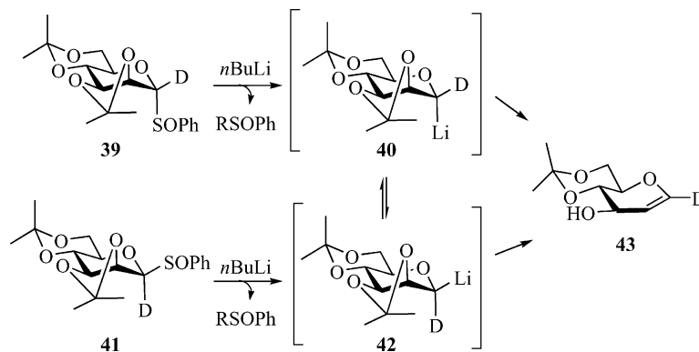
Scheme 10. Reactions of deuterated sulfoxides 39 and 41 with n BuLi.
