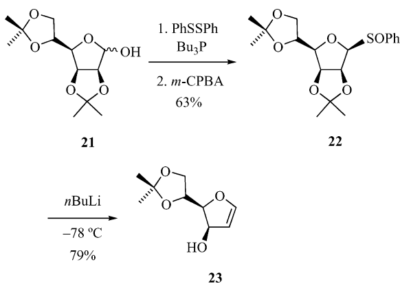
Scheme 6. Formation of furanoid glycal 23 by treatment of furanosyl sulfoxides 22 with n BuLi (3 equiv.) in THF at -78^\circ\text{C} .
