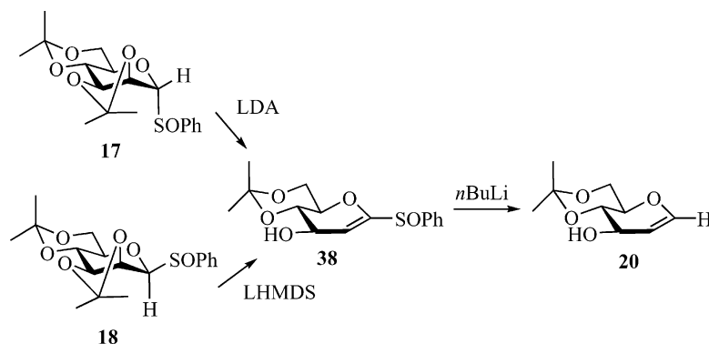
Scheme 9. Reaction of C-1-deuterated glycosyl sulfoxides with n BuLi to give deuterated glycol 20 .
