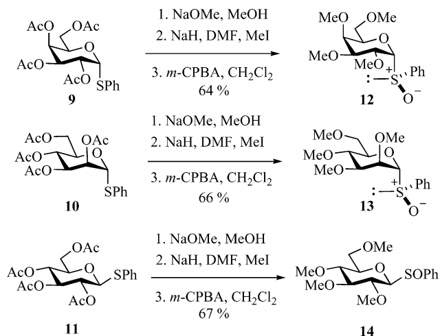
Scheme 3. Preparation of glycosyl sulfoxides.
