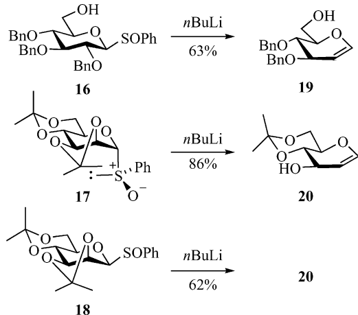
Scheme 5. Formation of glycals 19 and 20 by treatment of pyranosyl sulfoxides 16–18 with n BuLi in THF at -78^\circ\text{C} .
