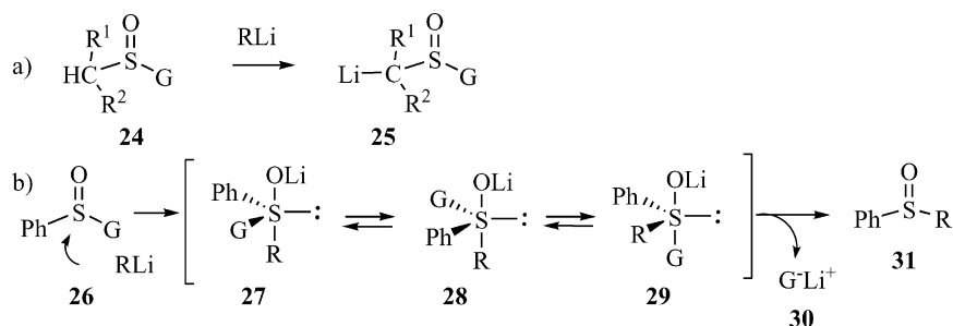
Scheme 7. Possible reaction pathways of reactions between sulfoxides and organolithium reagents.
