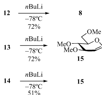
Scheme 4. Formation of glycals by treatment of pyranosyl sulfoxides with n BuLi (3 equiv.) in THF at -78^\circ\text{C} .
