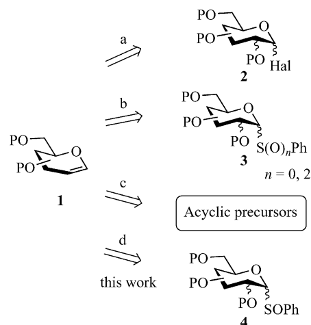
Scheme 1. Strategies for the synthesis of pyranoid glycals; P = protecting group.
